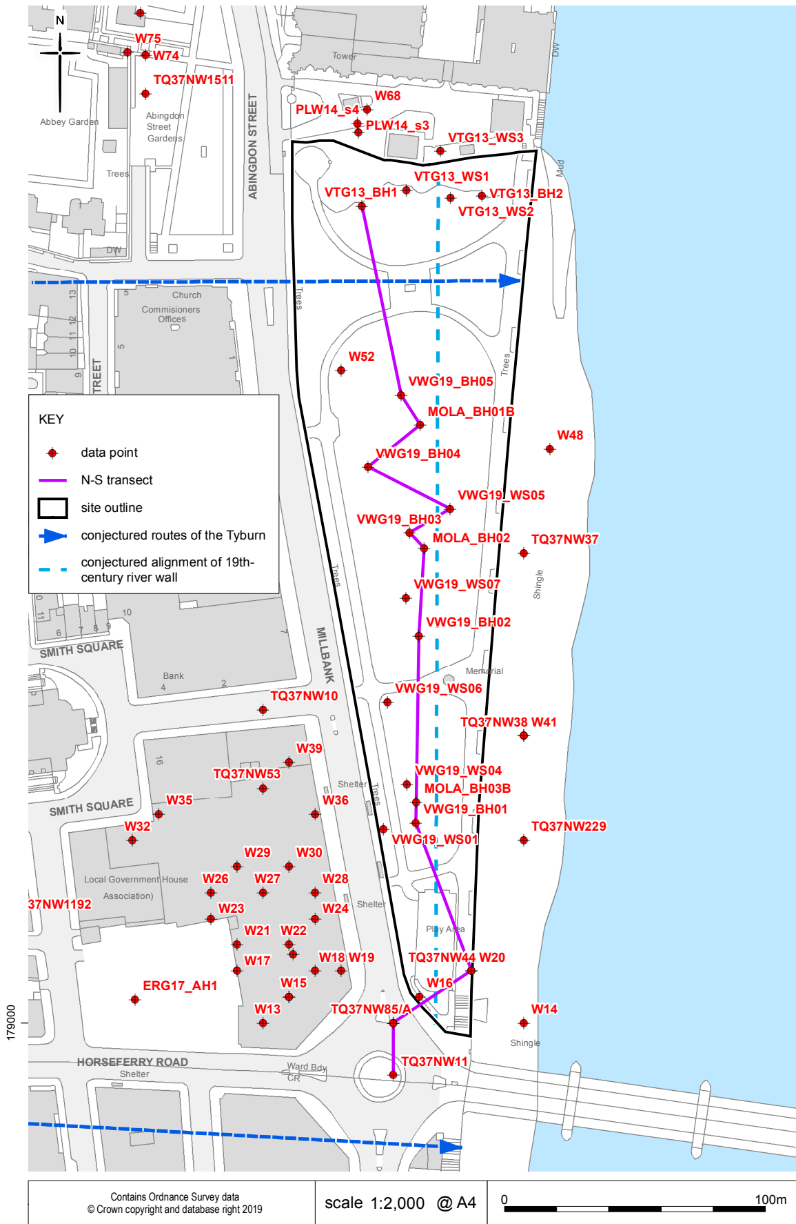
Fig 2 MOLA boreholes, geotechnical interventions and line of transect
