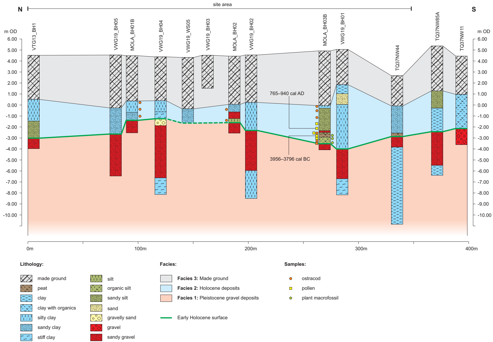
Fig 3 North to south transect across the site showing sample points within MOLA boreholes
