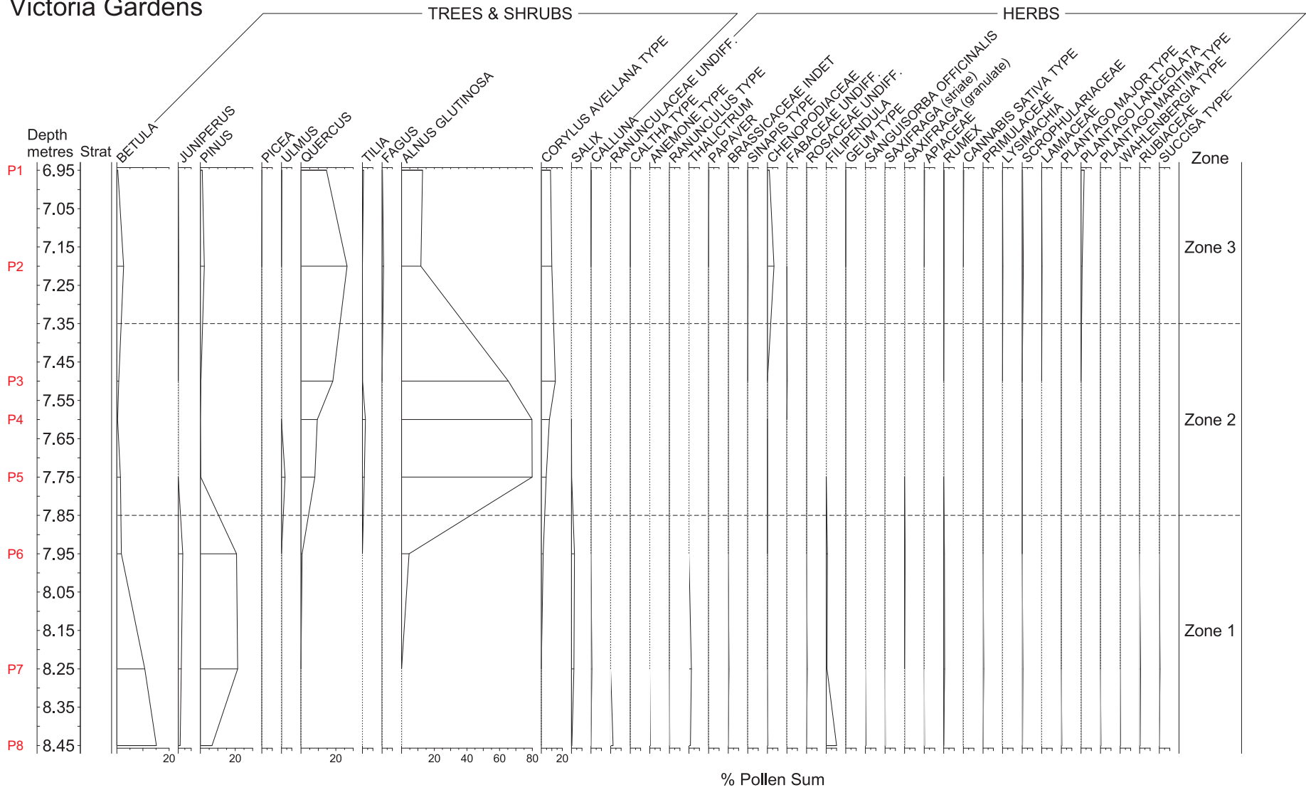
Fig 6 Pollen diagram
