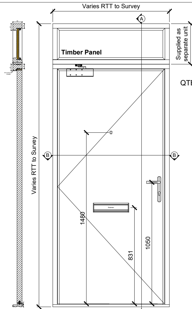
ELEVATION SCALE 1:20
