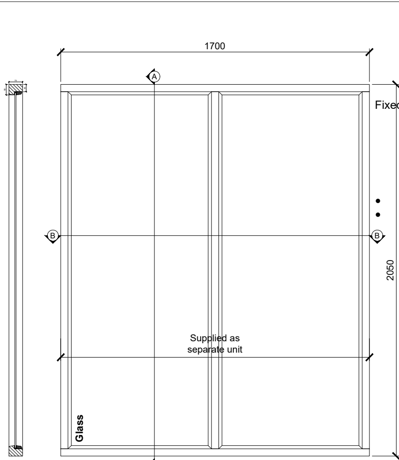
ELEVATION SCALE 1:20
